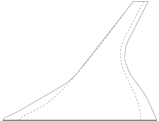
Fig. 28 Planform comparisons of the second-generation BWB with the Boeing Baseline BWB: —, Boeing Baseline and ---, second generation (scaled).
