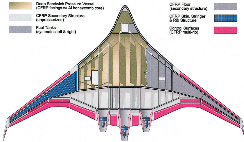
Fig. 20 Structural layout of second-generation BWB.
