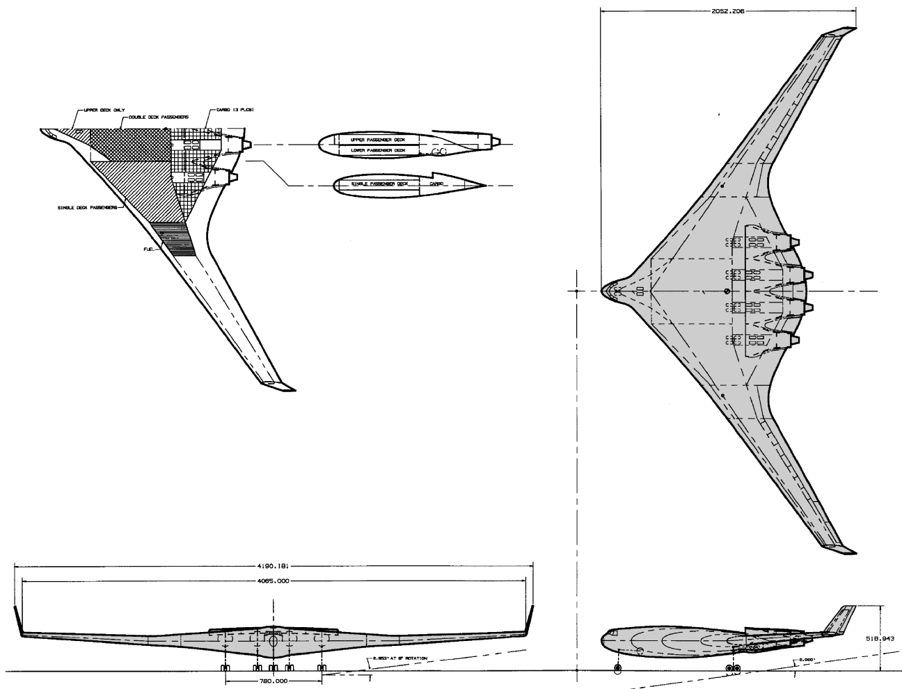
Fig. 6 First-generation BWB.
