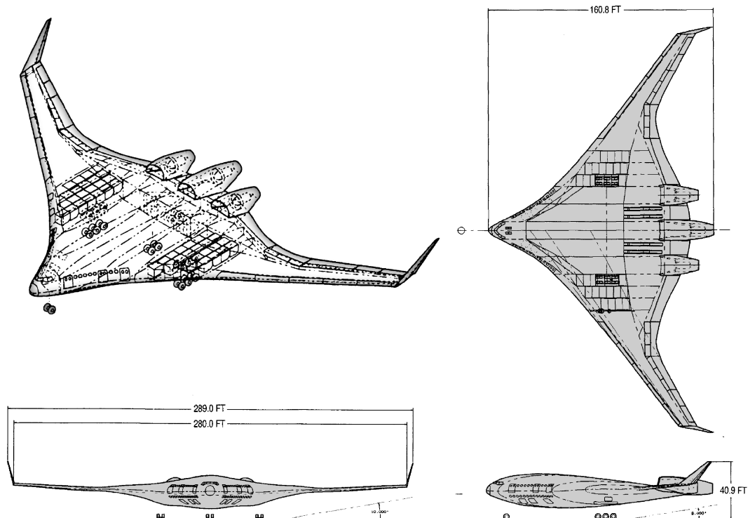
Fig. 9 Second-generation BWB.
